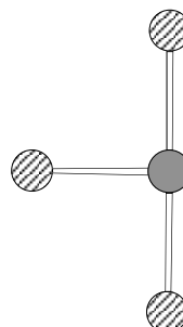
AX 3 E 2 T-shaped
