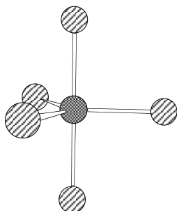
AX 5 Trigonal Bipyramidal
