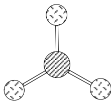
AX 3 Trigonal Planar
