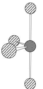
AX 4 E Seesaw
